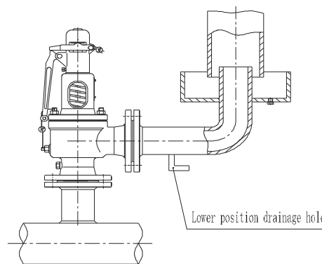
Fig. 6 For steam
