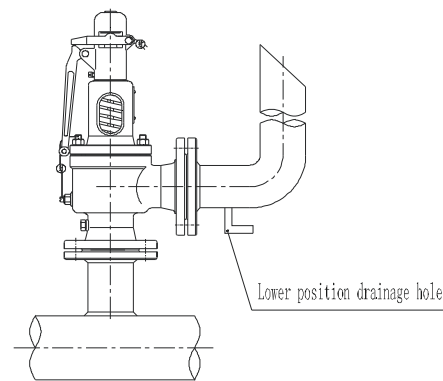
Fig. 6 For steam
